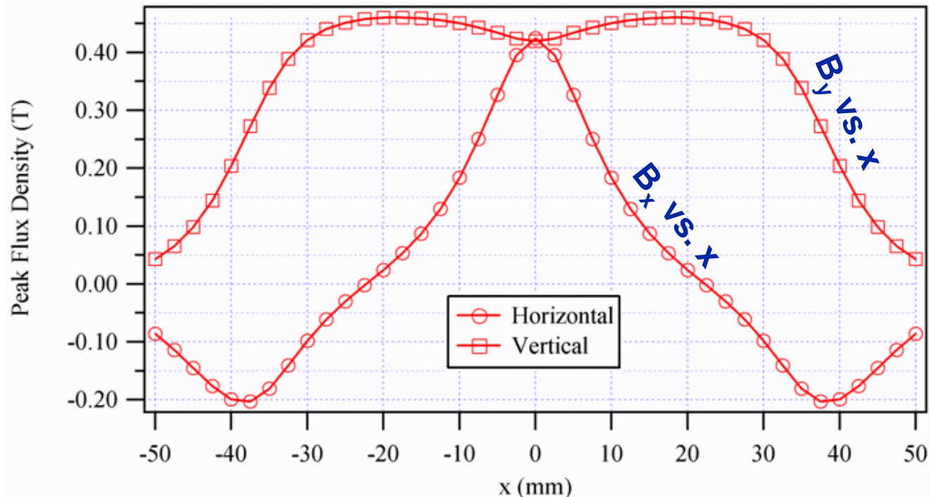
Figure 24. The transverse roll off for the Circular undulator phase.
