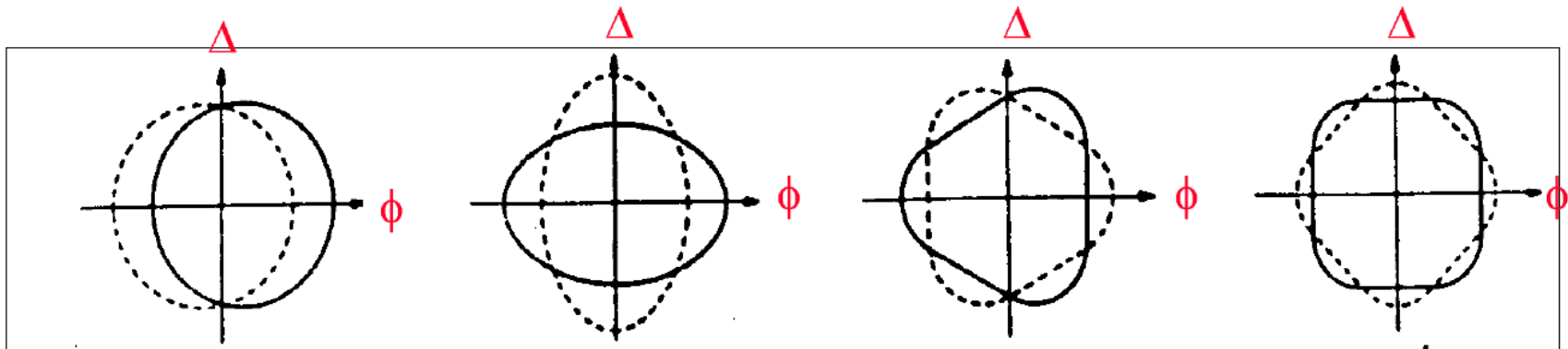
m = 1 dipole mode
