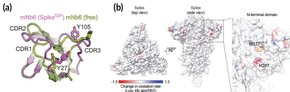
(a) Crystallography data from the ALS show atomic-level details of key Nb6 regions. (b) X-ray footprinting experiments performed at the ALS revealed a cluster of residues in the spike's N-terminal domain, where it likely interacts with Nb3.
