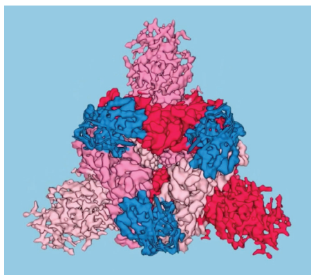
Top-down view of three nanobodies (blue) bound to the tip of the SARS-CoV-2 spike protein (red/pink). The nanobodies were engineered to be extremely effective at blocking the virus from entering a host cell.
